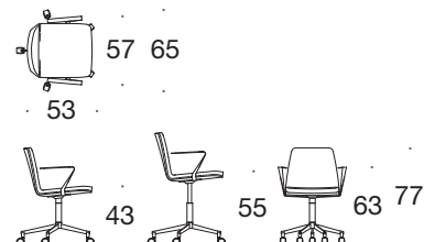
5-star, high back, armrests
